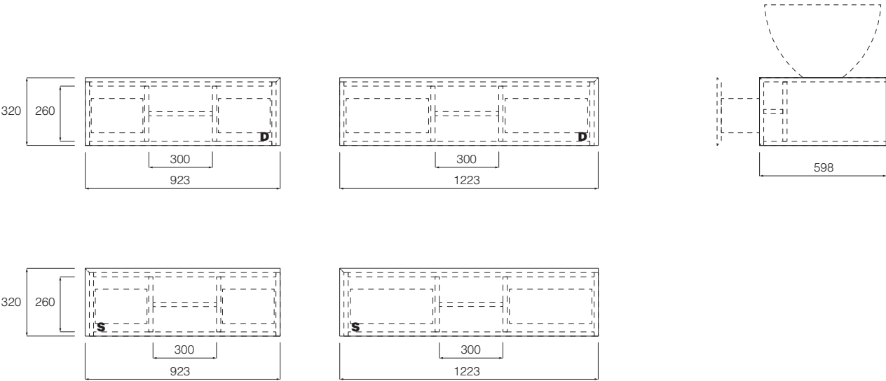
Base unit for washbasin with drawer - MIDDLE USE
