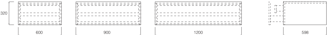
MIDDLE-USE base unit with drawer + internal drawer.
