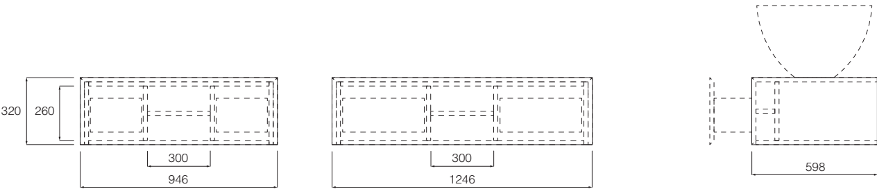
Base unit for washbasin with drawer - END USE
