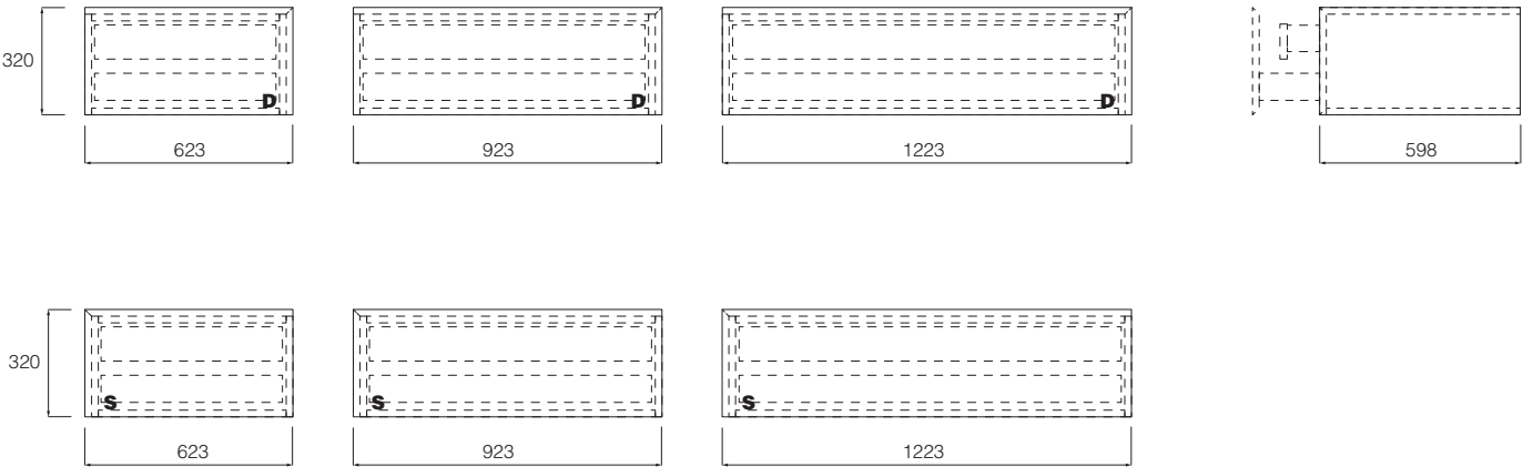
MIDDLE-USE base unit with drawer + internal drawer.
