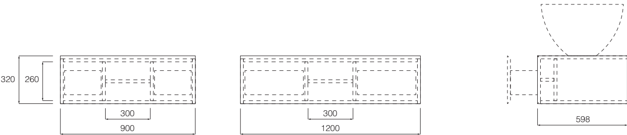
Base unit for washbasin with drawer - MIDDLE USE
