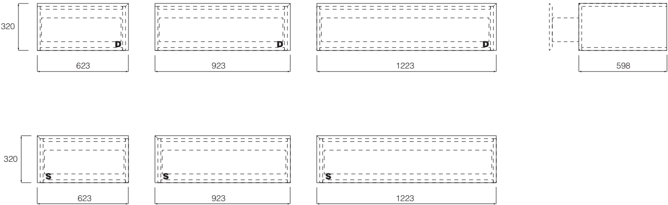
MIDDLE-USE base unit with drawer.
