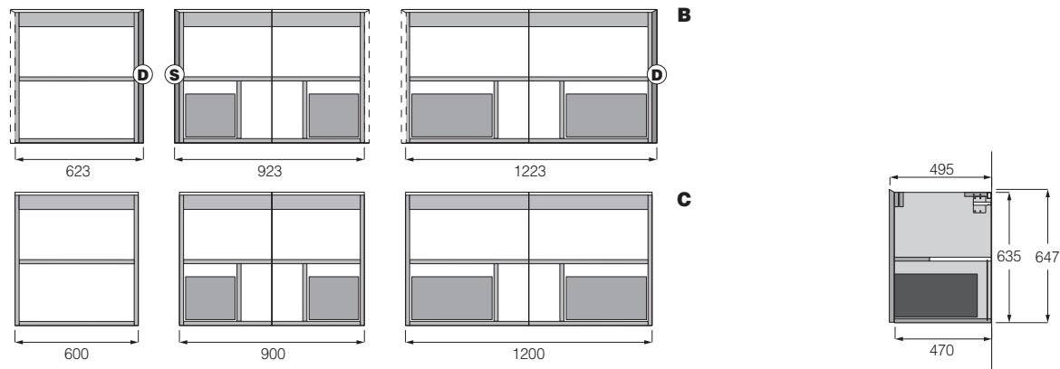
Storage base units with hinged door. - H 612 mm
