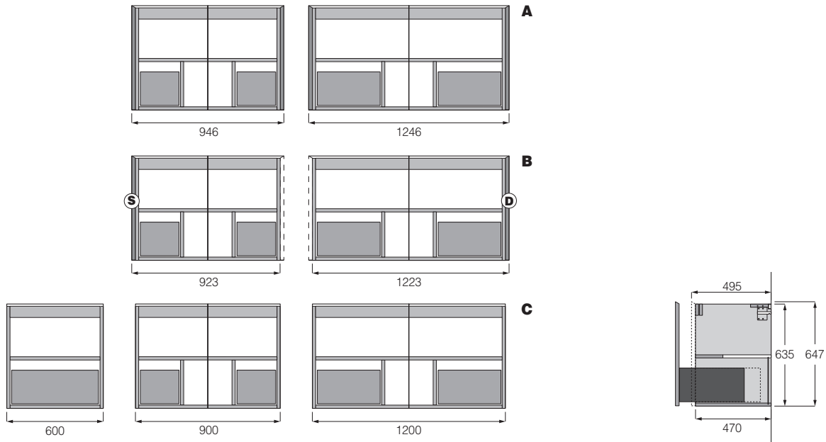
Base units for washbasin with pull-out doors in FINISH. - H 612 mm
