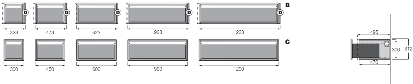
Storage base units with drawer. - H 312 mm
