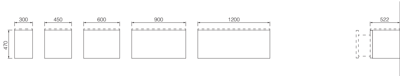
Base unit with drawer + internal drawer.
