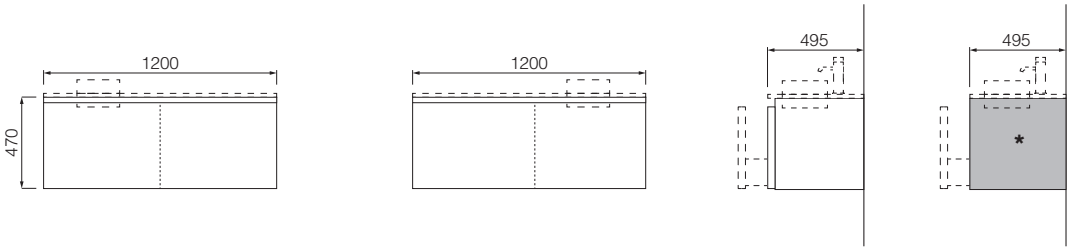
Single front base unit for washbasin with double drawer + 1 internal drawer
