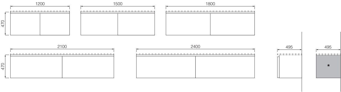
Base unit for washbasin with 2 coplanar sliding doors
