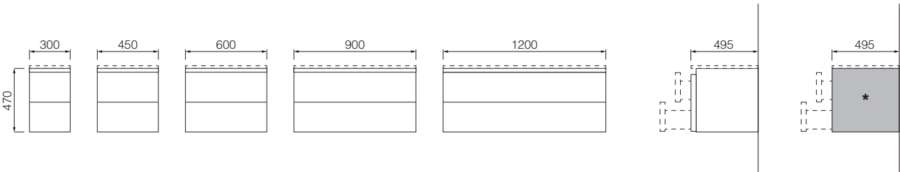
Base unit with 2 drawers
