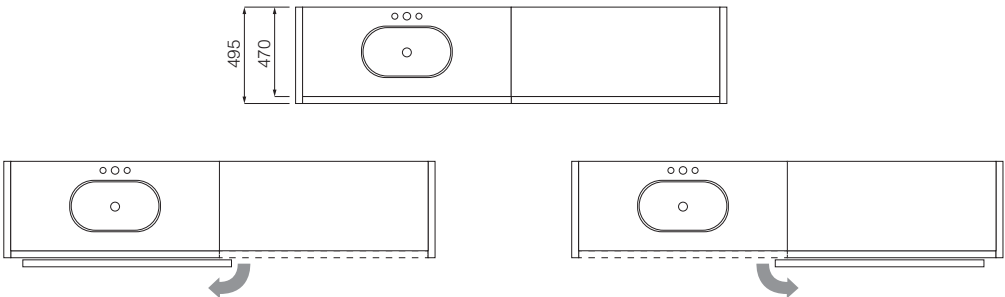
Base unit with 2 coplanar doors - DOOR OPENING
